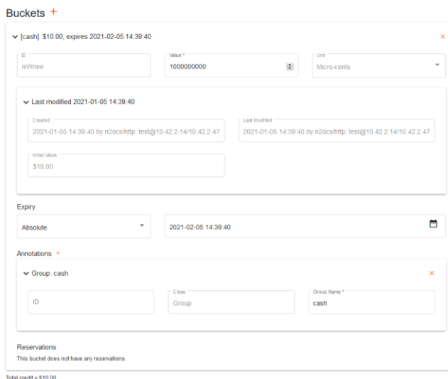
Figure 2 OCS Bucket Management
